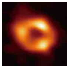
©EHT Collaboration
